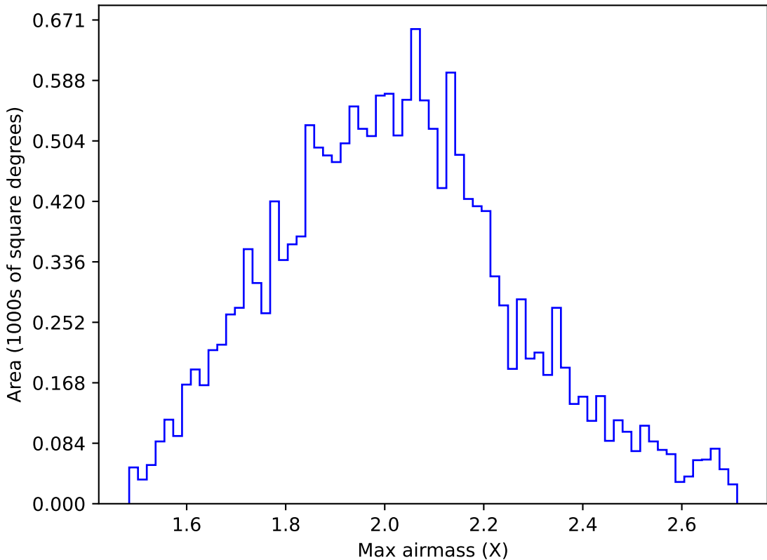
internal_u_expt45_nscale1.1v3.4_10yrs WFD g band: Max airmass
