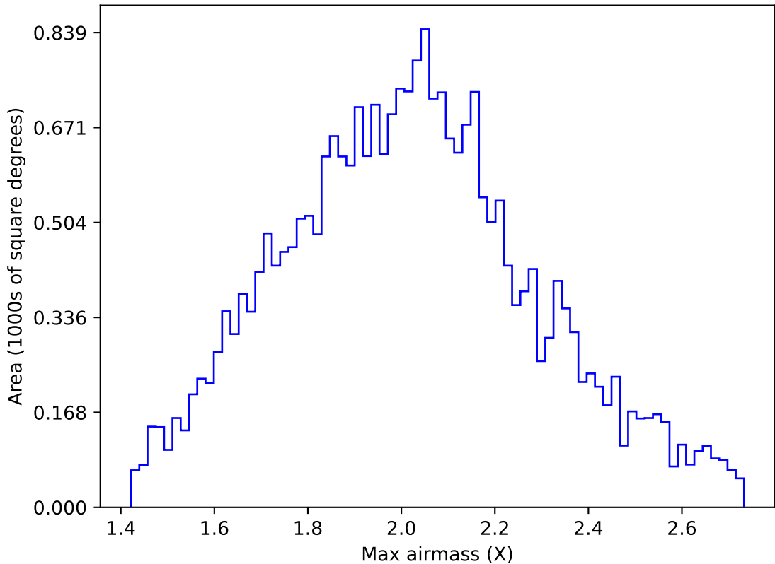
internal_u_expt45_nscale1.1v3.4_10yrs All sky g band: Max airmass
