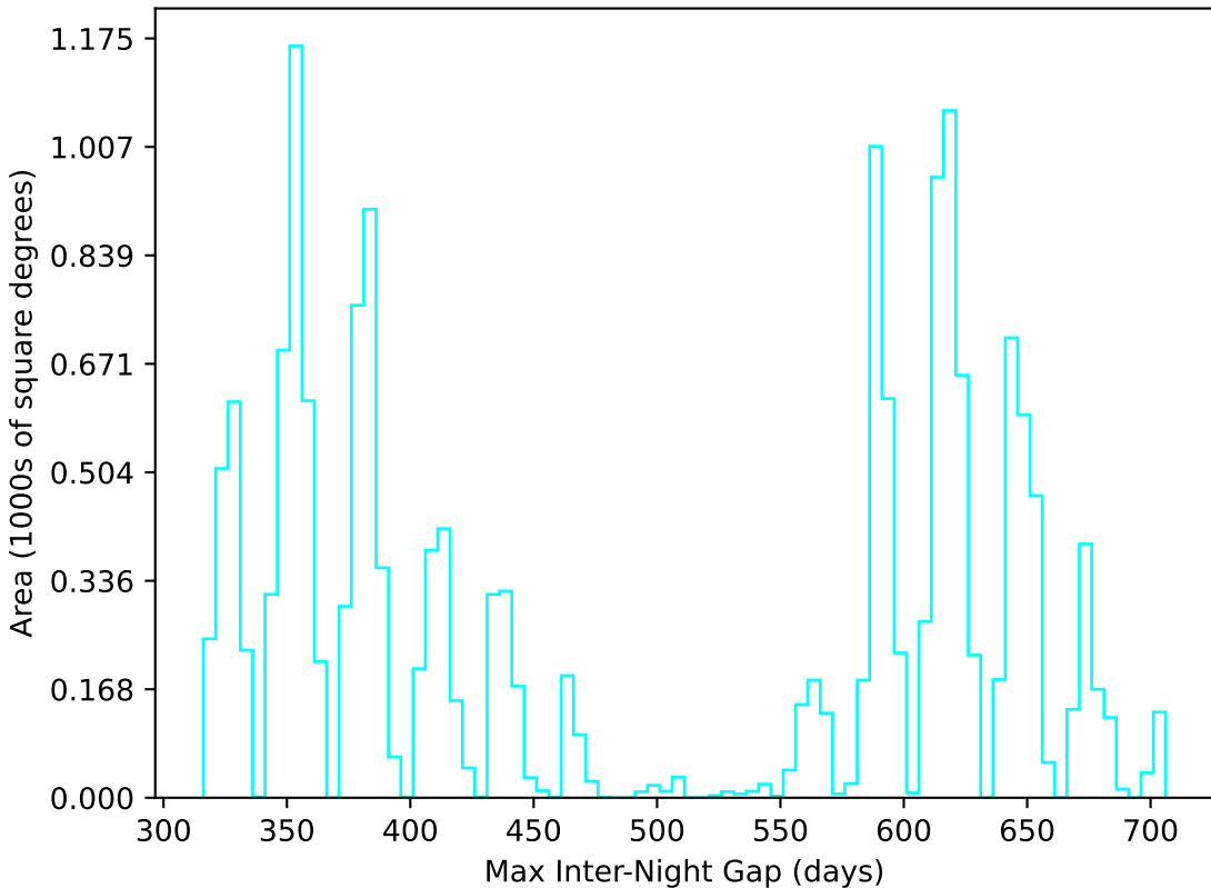
internal_u_expt45_nscale1.1v3.4_10yrs WFD u band: Max Inter-Night Gap
