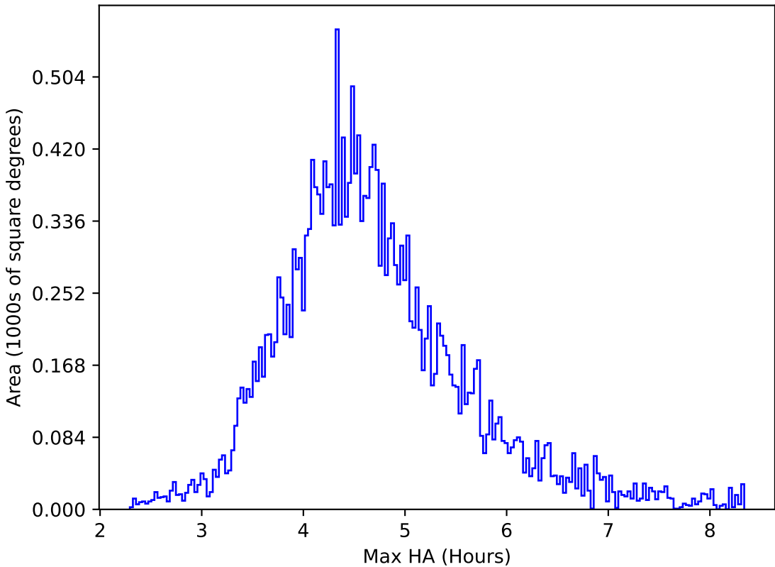
internal_u_expt45_nscale1.1v3.4_10yrs All sky y band: Max HA
