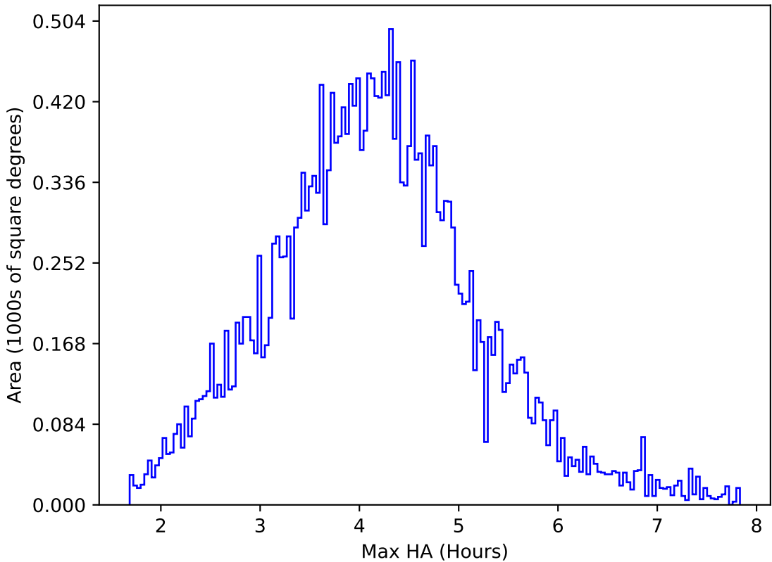
internal_u_expt45_nscale1.1v3.4_10yrs All sky r band: Max HA
