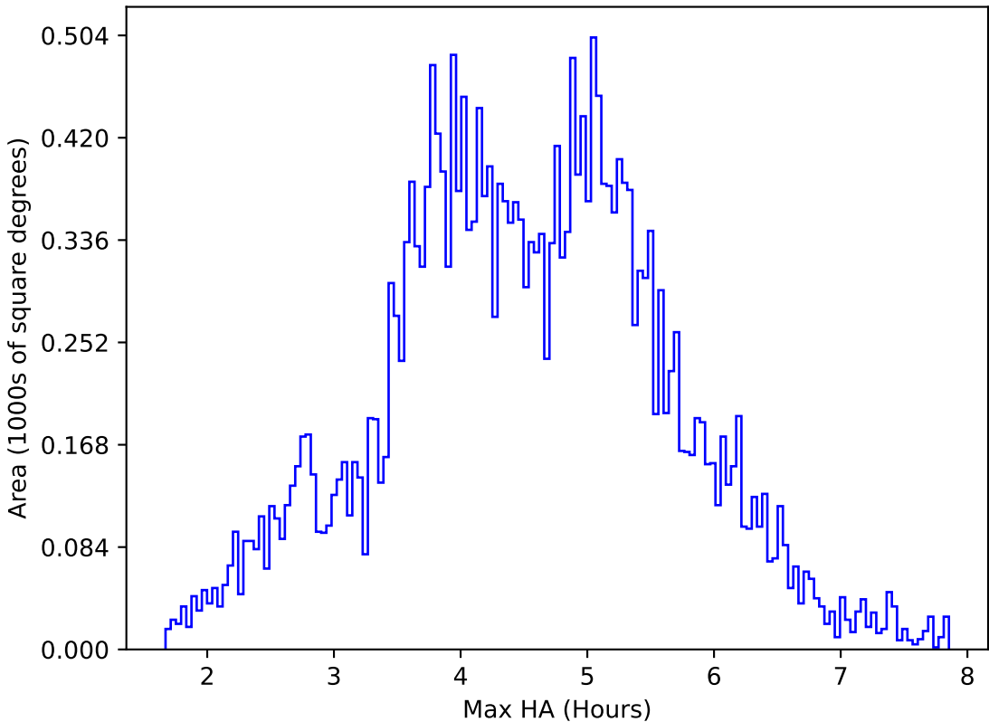
internal_u_expt45_nscale1.1v3.4_10yrs All sky i band: Max HA
