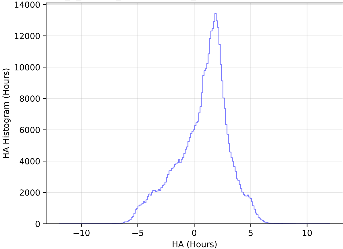
internal_u_expt45_nscale1.1v3.4_10yrs WFD z band: HA Histogram
