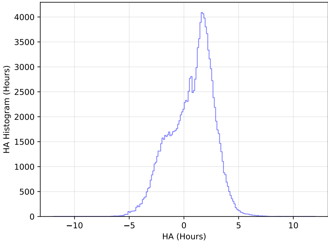
internal_u_expt45_nscale1.1v3.4_10yrs WFD u band: HA Histogram
