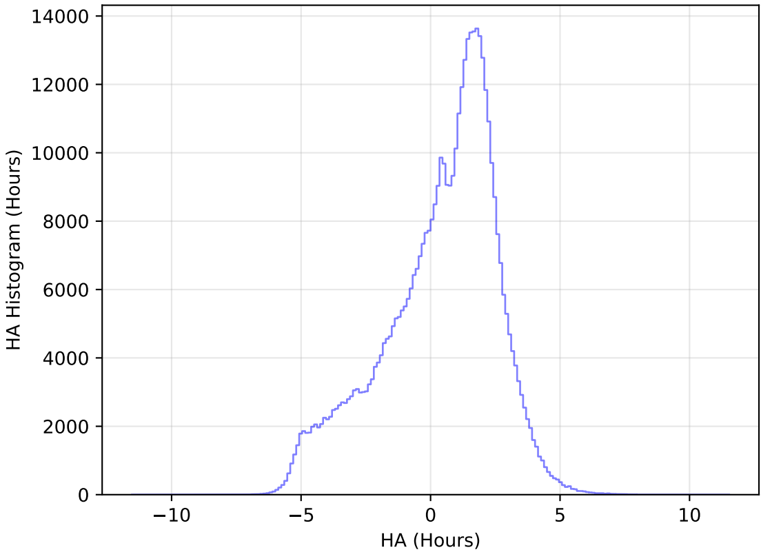
internal_u_expt45_nscale1.1v3.4_10yrs WFD r band: HA Histogram
