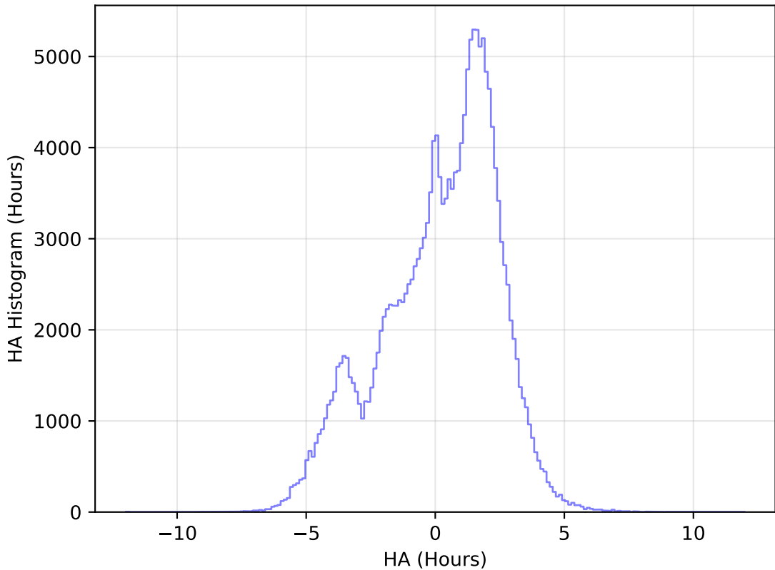
internal_u_expt45_nscale1.1v3.4_10yrs WFD g band: HA Histogram
