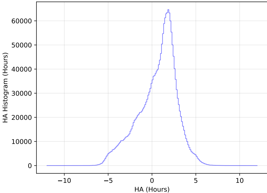
internal_u_expt45_nscale1.1v3.4_10yrs WFD all bands: HA Histogram
