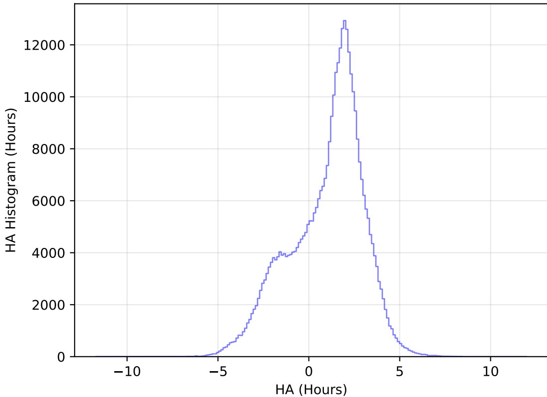
internal_u_expt45_nscale1.1v3.4_10yrs All sky y band: HA Histogram
