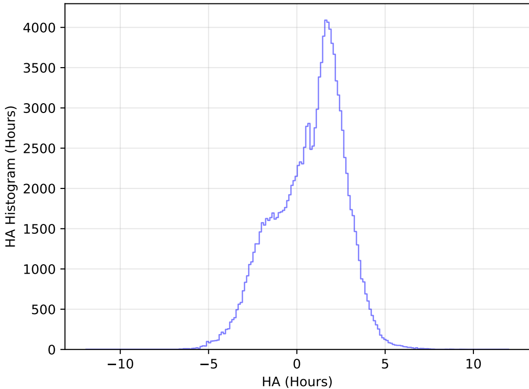
internal_u_expt45_nscale1.1v3.4_10yrs All sky u band: HA Histogram
