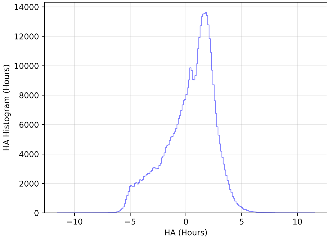
internal_u_expt45_nscale1.1v3.4_10yrs All sky r band: HA Histogram
