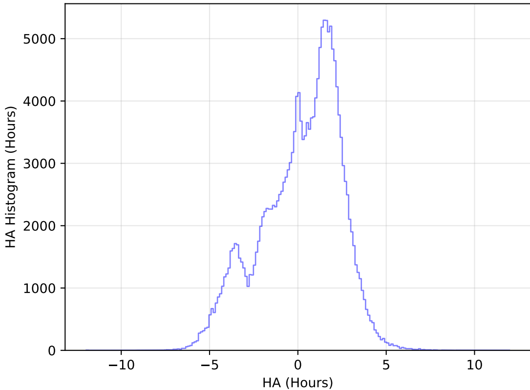
internal_u_expt45_nscale1.1v3.4_10yrs All sky g band: HA Histogram
