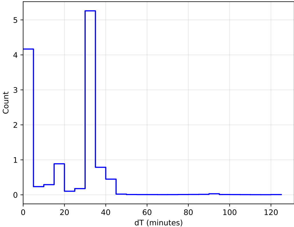
internal_u_expt45_nscale1.1v3.4_10yrs All sky: DeltaT Histogram
