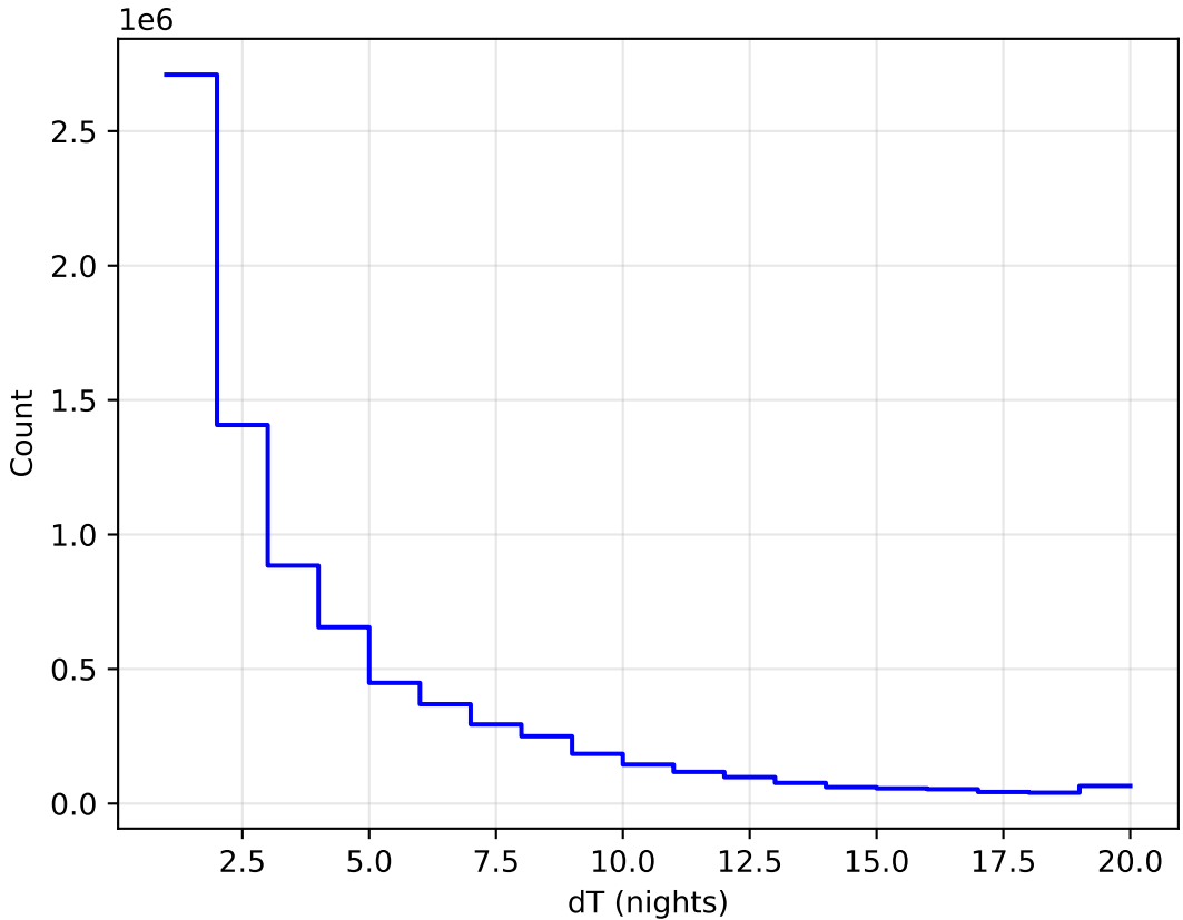
internal_u_expt45_nscale1.1v3.4_10yrs WFD all bands: DeltaNight Histogram
