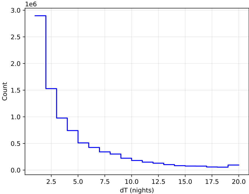
internal_u_expt45_nscale1.1v3.4_10yrs All sky all bands: DeltaNight Histogram
