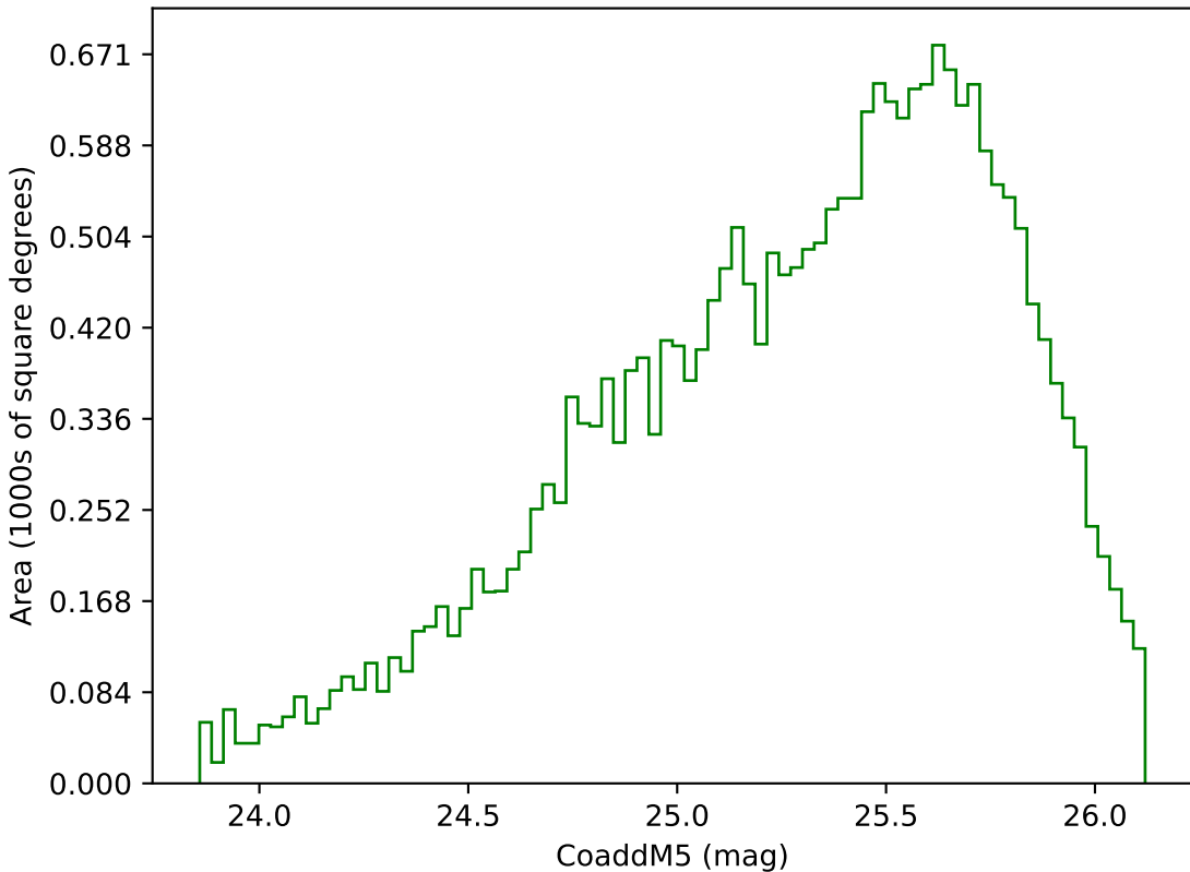
internal_u_expt45_nscale1.1v3.4_10yrs Yr 3-4 g band: CoaddM5
