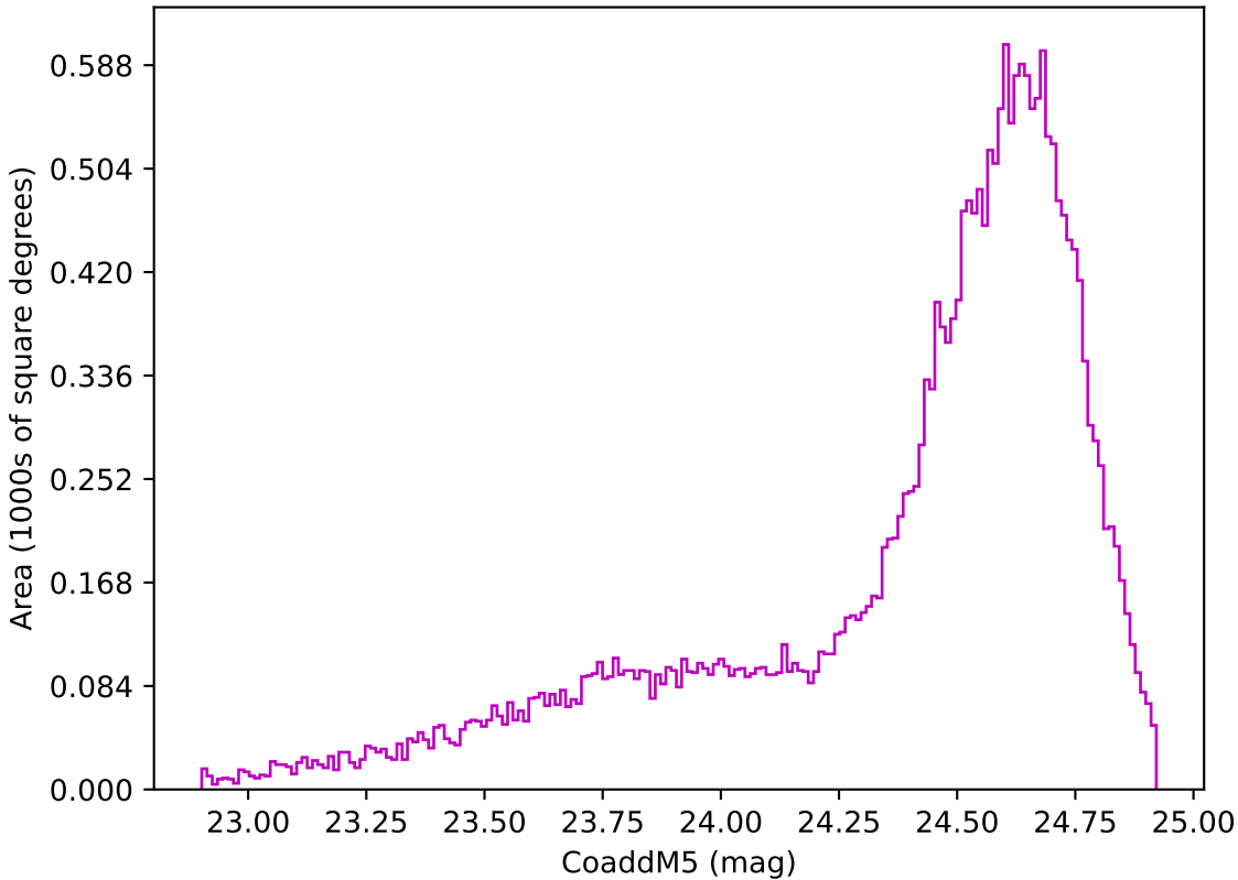
internal_u_expt45_nscale1.1v3.4_10yrs Yr 1 z band: CoaddM5
