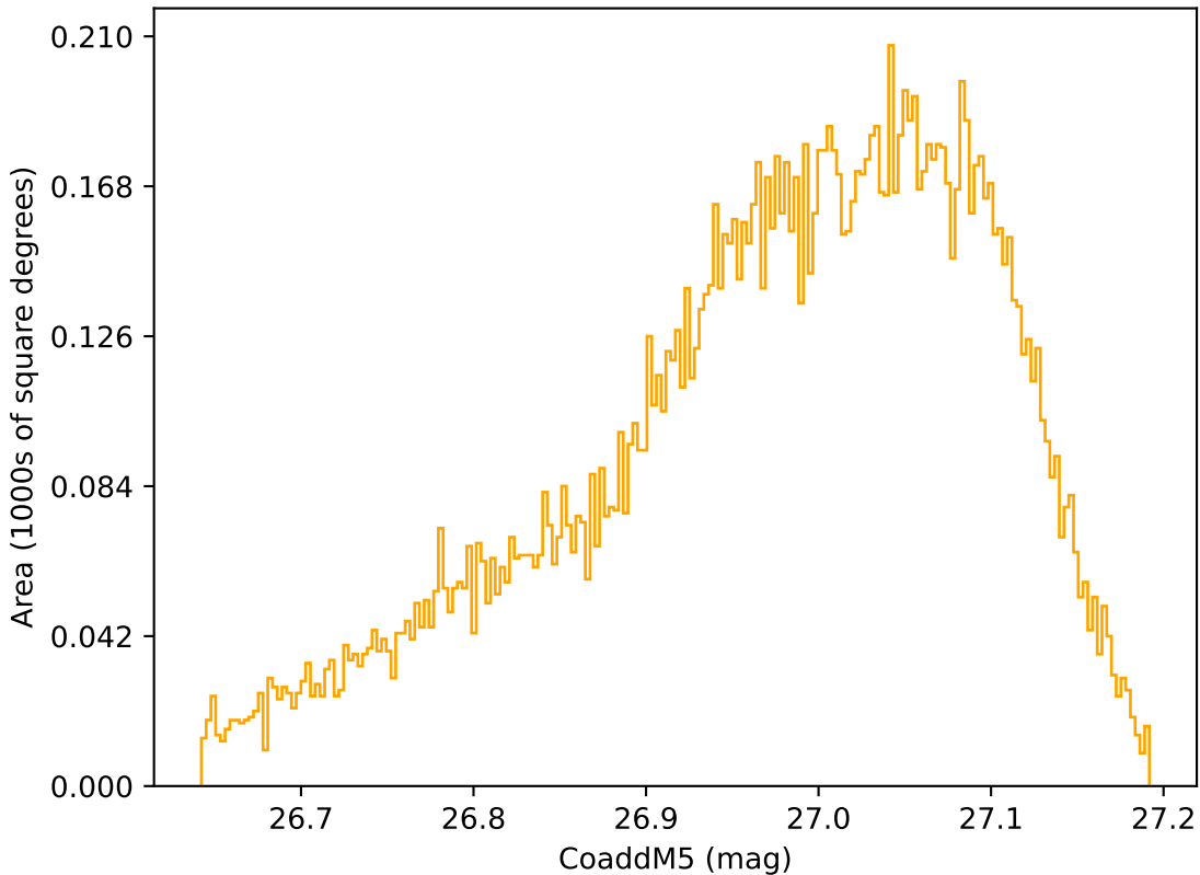
internal_u_expt45_nscale1.1v3.4_10yrs WFD r band: CoaddM5
