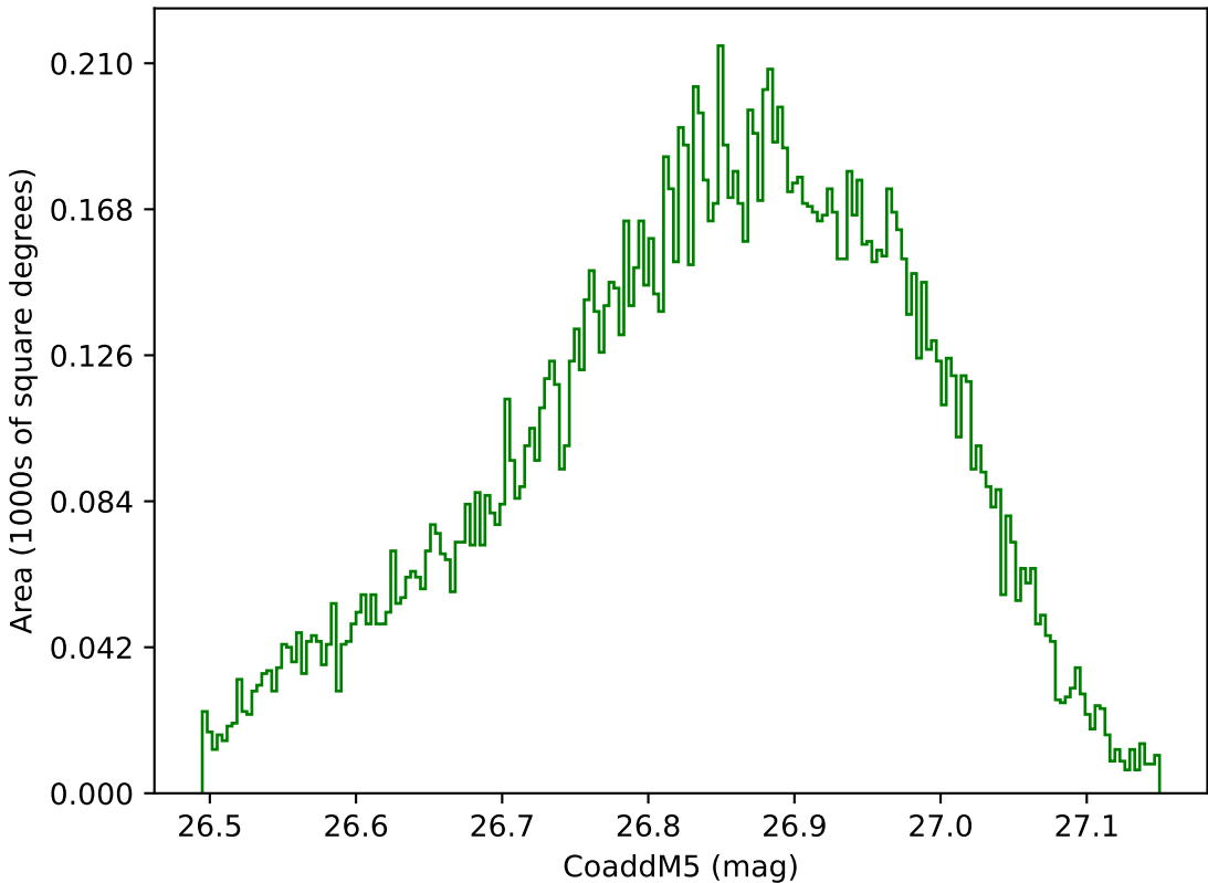
internal_u_expt45_nscale1.1v3.4_10yrs WFD g band: CoaddM5
