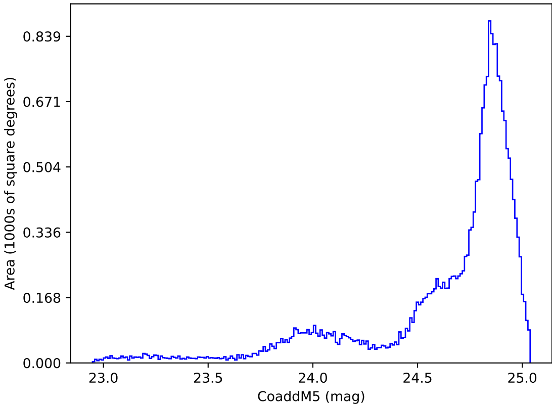
internal_u_expt45_nscale1.1v3.4_10yrs All sky y band: CoaddM5
