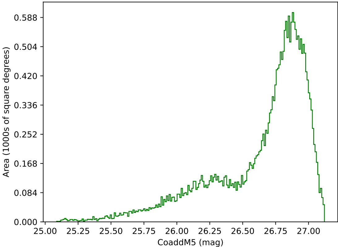
internal_u_expt45_nscale1.1v3.4_10yrs All sky g band: CoaddM5
