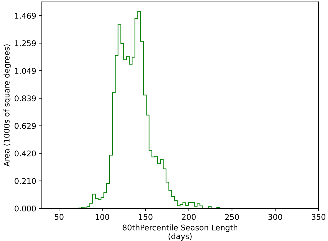
internal_u_expt45_nscale1.1v3.4_10yrs WFD g band: 80thPercentile Season Length
