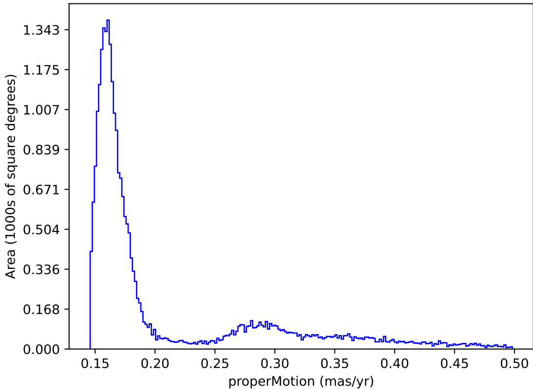
internal_u_expt45_nscale1.1v3.4_10yrs : properMotion
