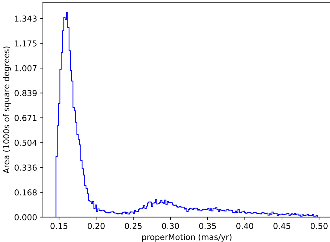
internal_u_expt45_nscale1.1v3.4_10yrs : properMotion
