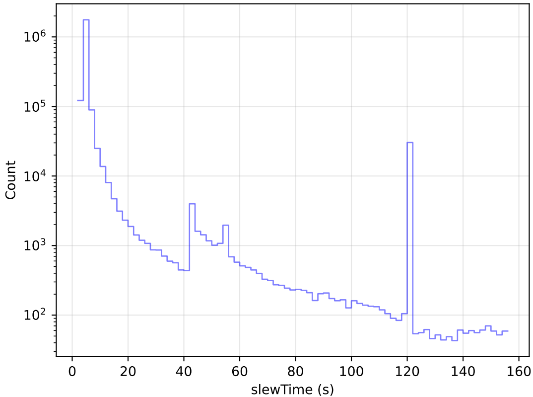
internal_u_expt45_nscale1.1v3.4_10yrs All visits: Slew Time Histogram
