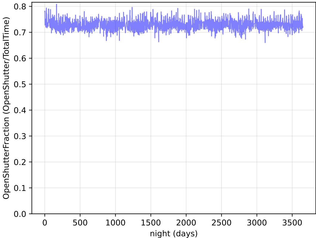
internal_u_expt45_nscale1.1v3.4_10yrs : OpenShutterFraction
