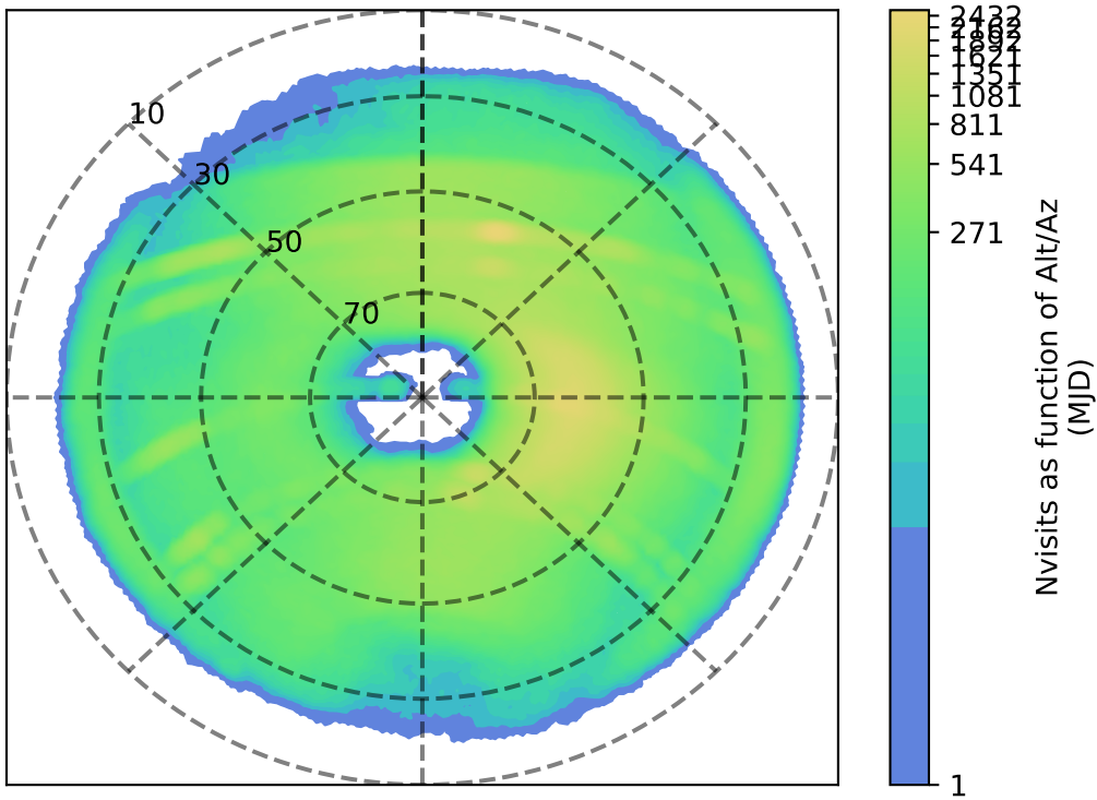
internal_u_expt45_nscale1.1v3.4_10yrs z: Nvisits as function of Alt/Az
