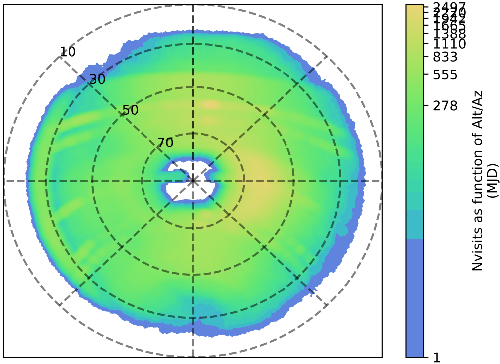
internal_u_expt45_nscale1.1v3.4_10yrs r: Nvisits as function of Alt/Az
