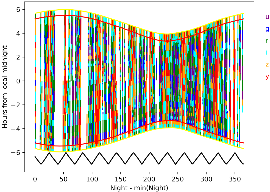
internal_u_expt45_nscale1.1v3.4_10yrs year 4-5: Hourglass
