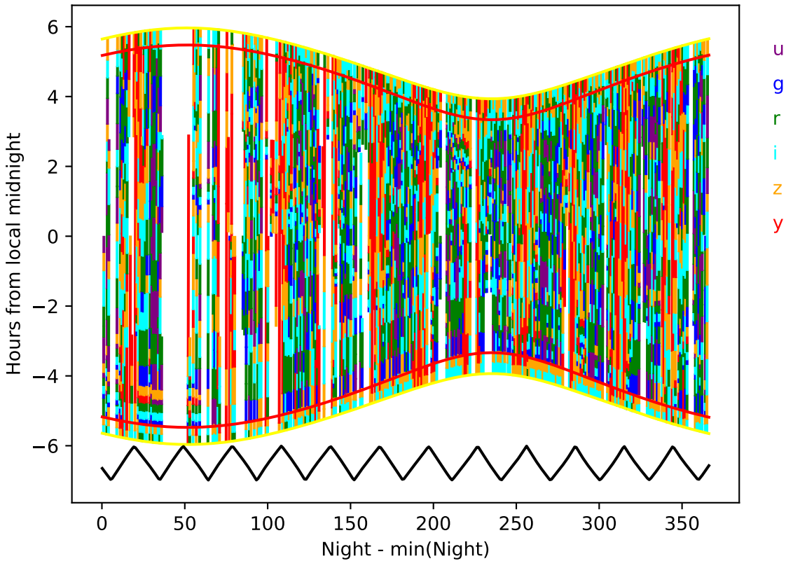
internal_u_expt45_nscale1.1v3.4_10yrs year 2-3: Hourglass
