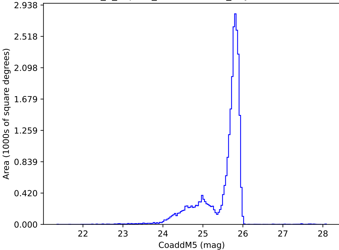
internal_u_expt45_nscale1.1v3.4_10yrs z: CoaddM5
