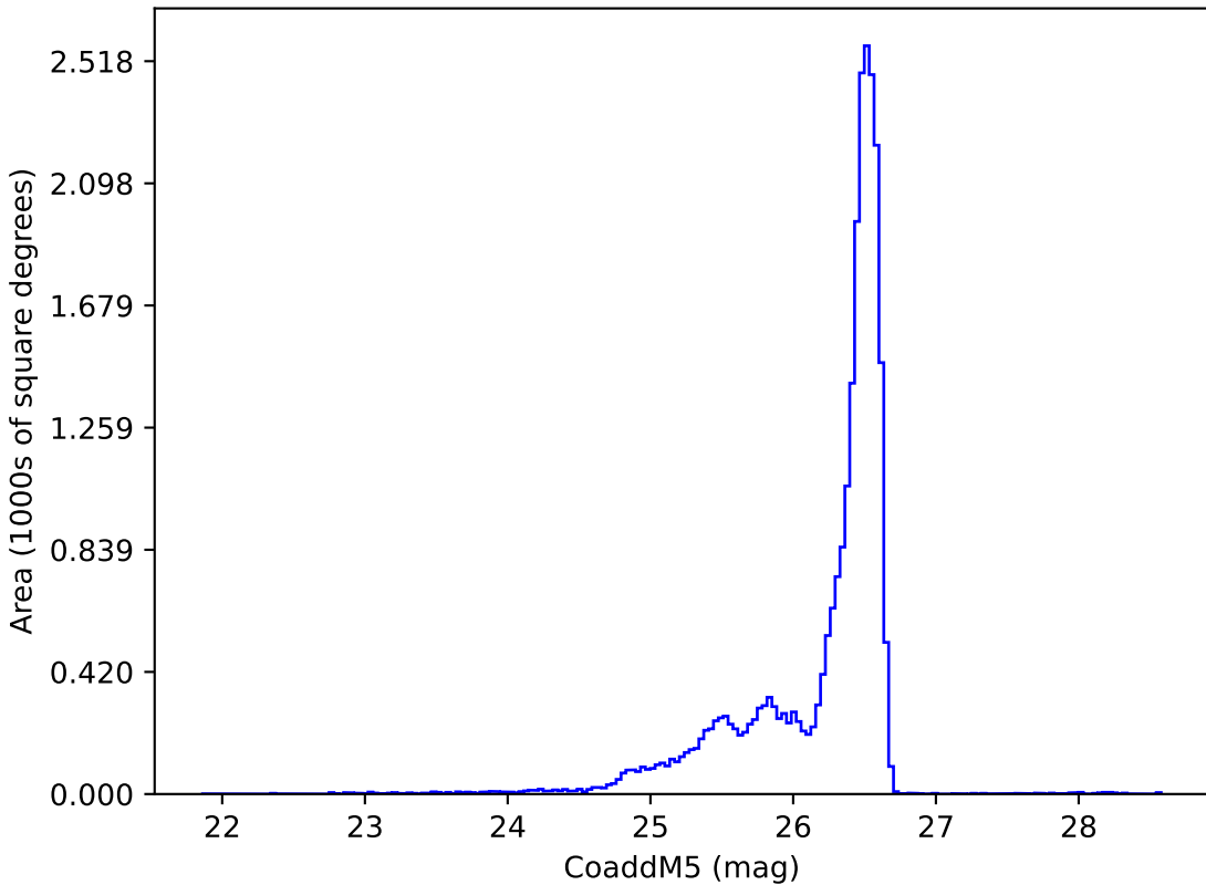
internal_u_expt45_nscale1.1v3.4_10yrs i: CoaddM5
