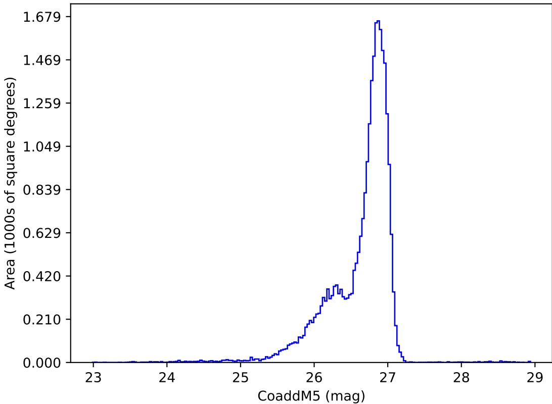
internal_u_expt45_nscale1.1v3.4_10yrs g: CoaddM5
