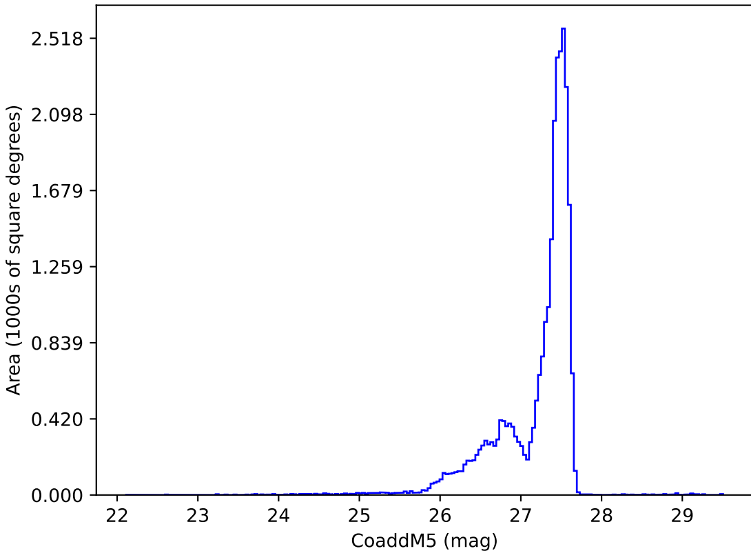
internal_u_expt45_nscale1.1v3.4_10yrs : CoaddM5
