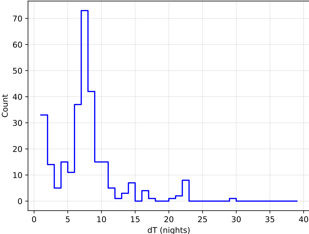
internal_u_expt45_nscale1.1v3.4_10yrs all bands: DD:EDFS Delta Nights Histogram
