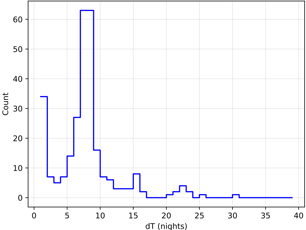
internal_u_expt45_nscale1.1v3.4_10yrs all bands: DD:ECDFS Delta Nights Histogram
