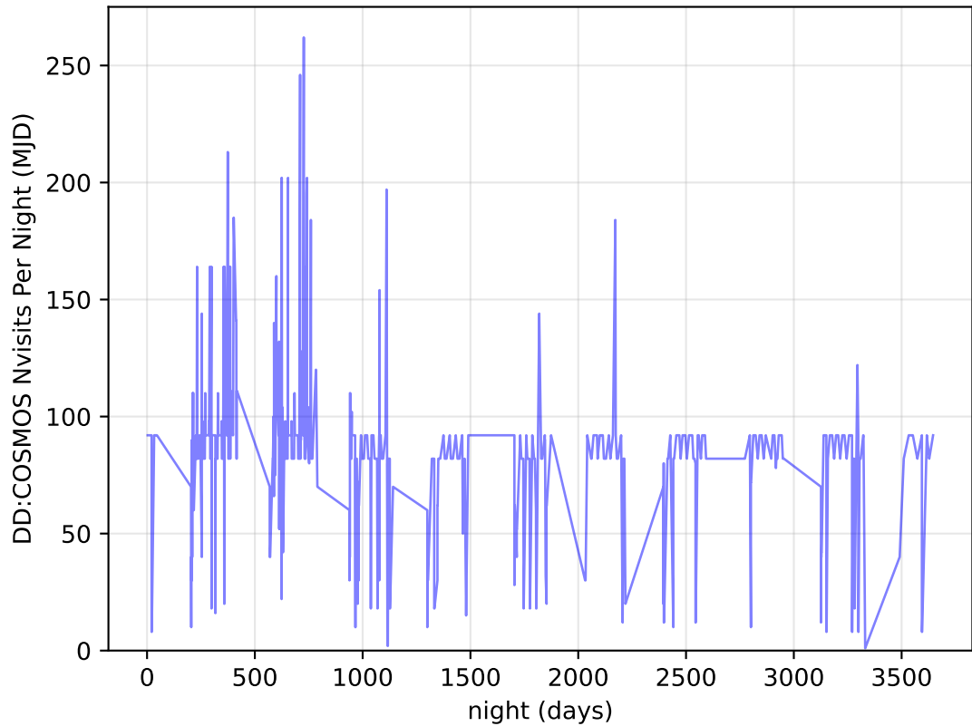
internal_u_expt45_nscale1.1v3.4_10yrs all bands: DD: COSMOS Nvisits Per Night
