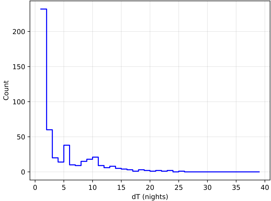
internal_u_expt45_nscale1.1v3.4_10yrs all bands: DD:COSMOS Delta Nights Histogram
