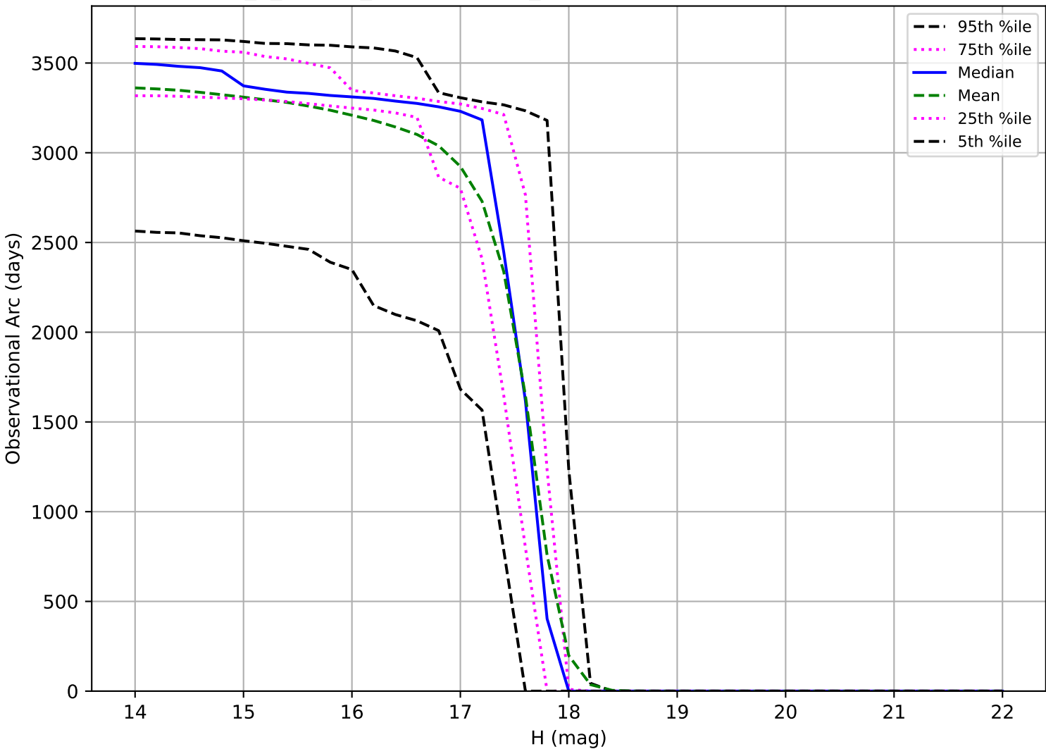
internal_u_expt45_nscale1.0v3.4_10yrs: Observational Arc Length Trojan
