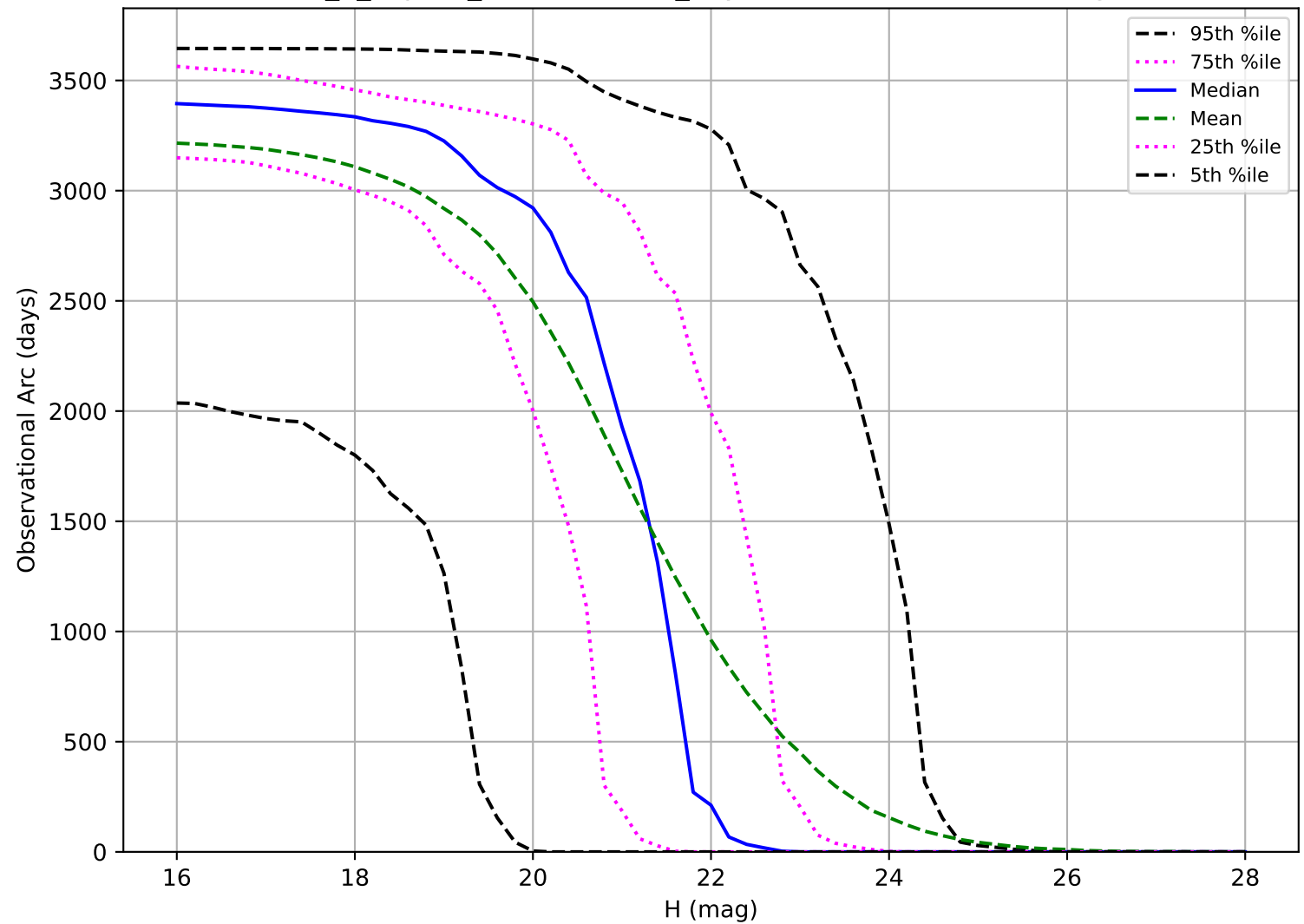
internal_u_expt45_nscale1.0v3.4_10yrs: Observational Arc Length PHA
