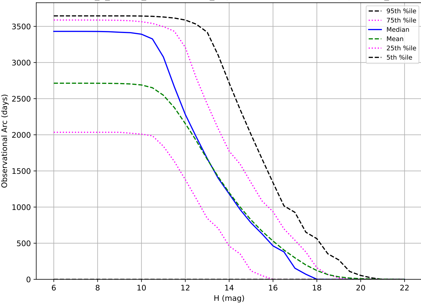
internal_u_expt45_nscale1.0v3.4_10yrs: Observational Arc Length OCC_r5
