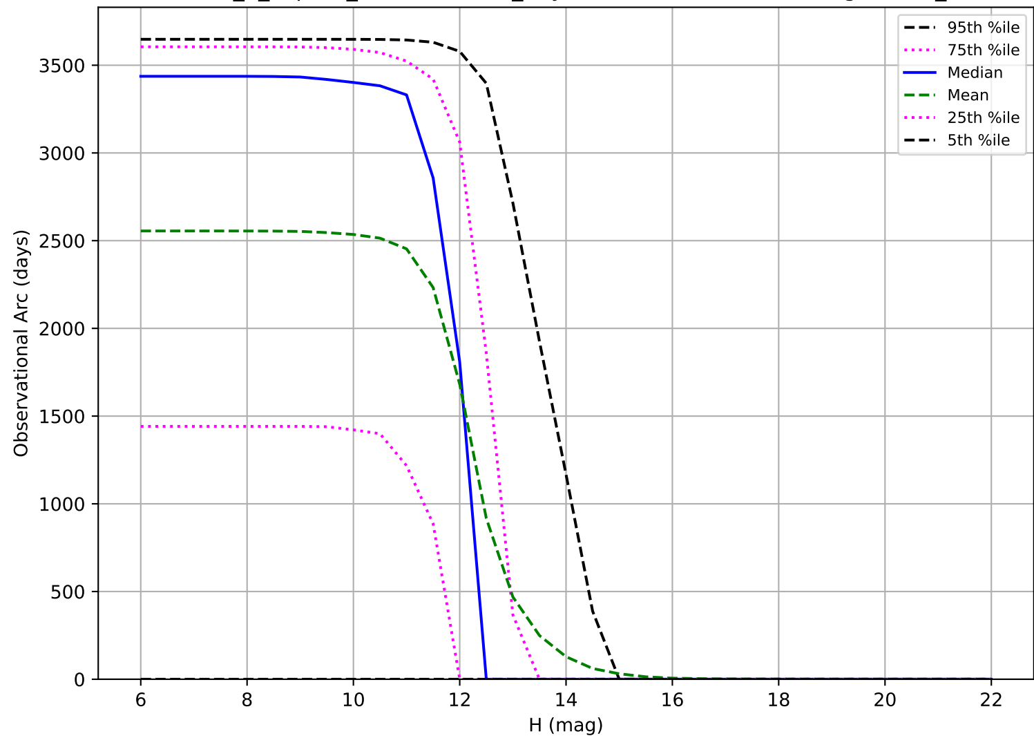
internal_u_expt45_nscale1.0v3.4_10yrs: Observational Arc Length OCC_r20
