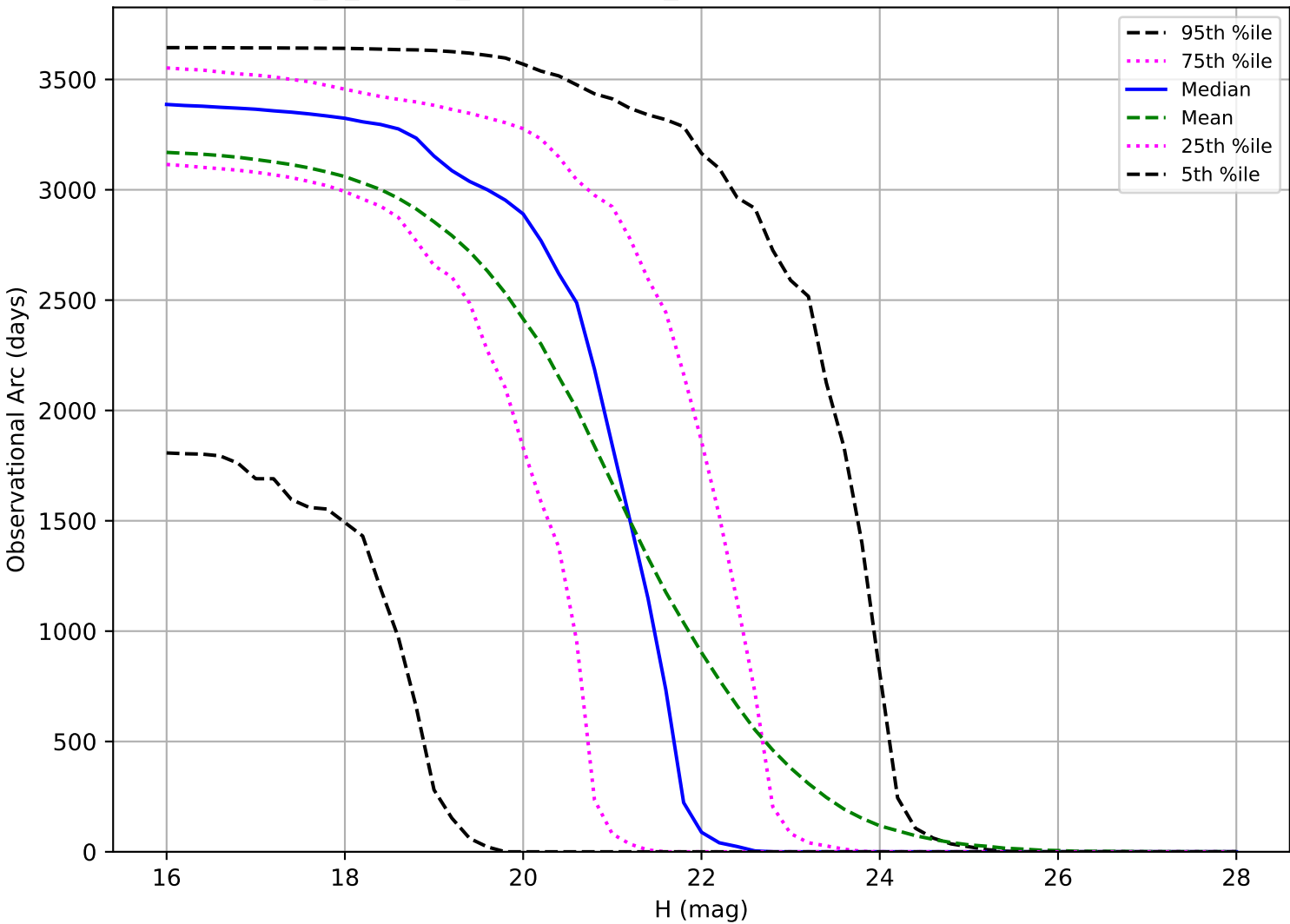
internal_u_expt45_nscale1.0v3.4_10yrs: Observational Arc Length NEO
