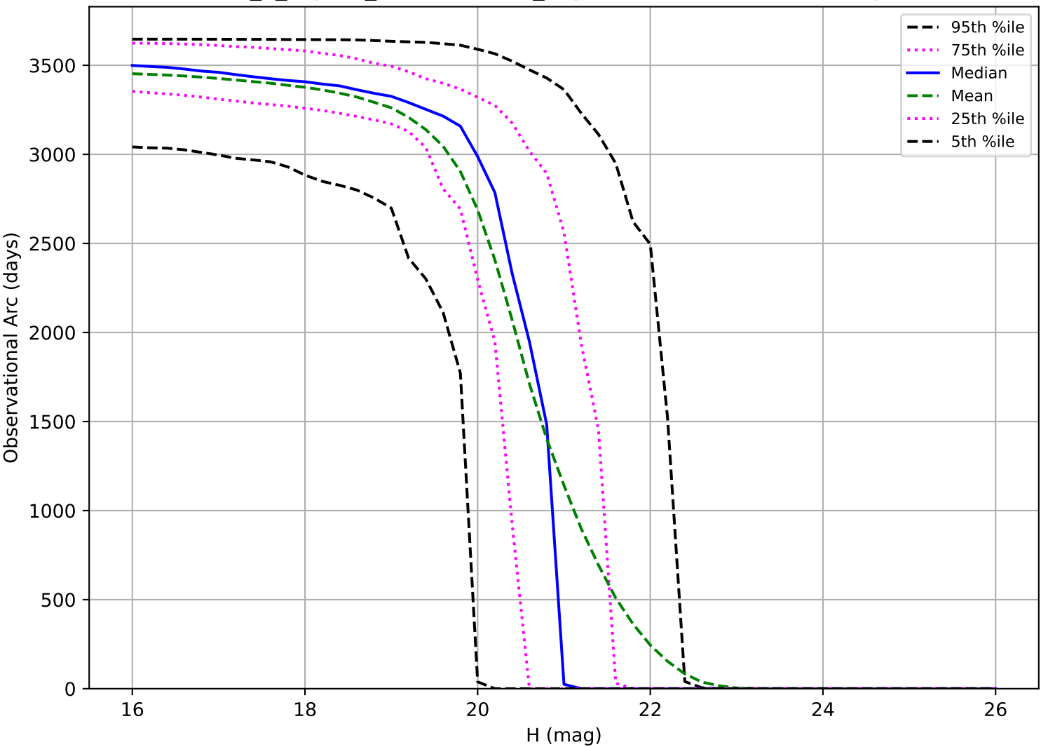
internal_u_expt45_nscale1.0v3.4_10yrs: Observational Arc Length MBA
