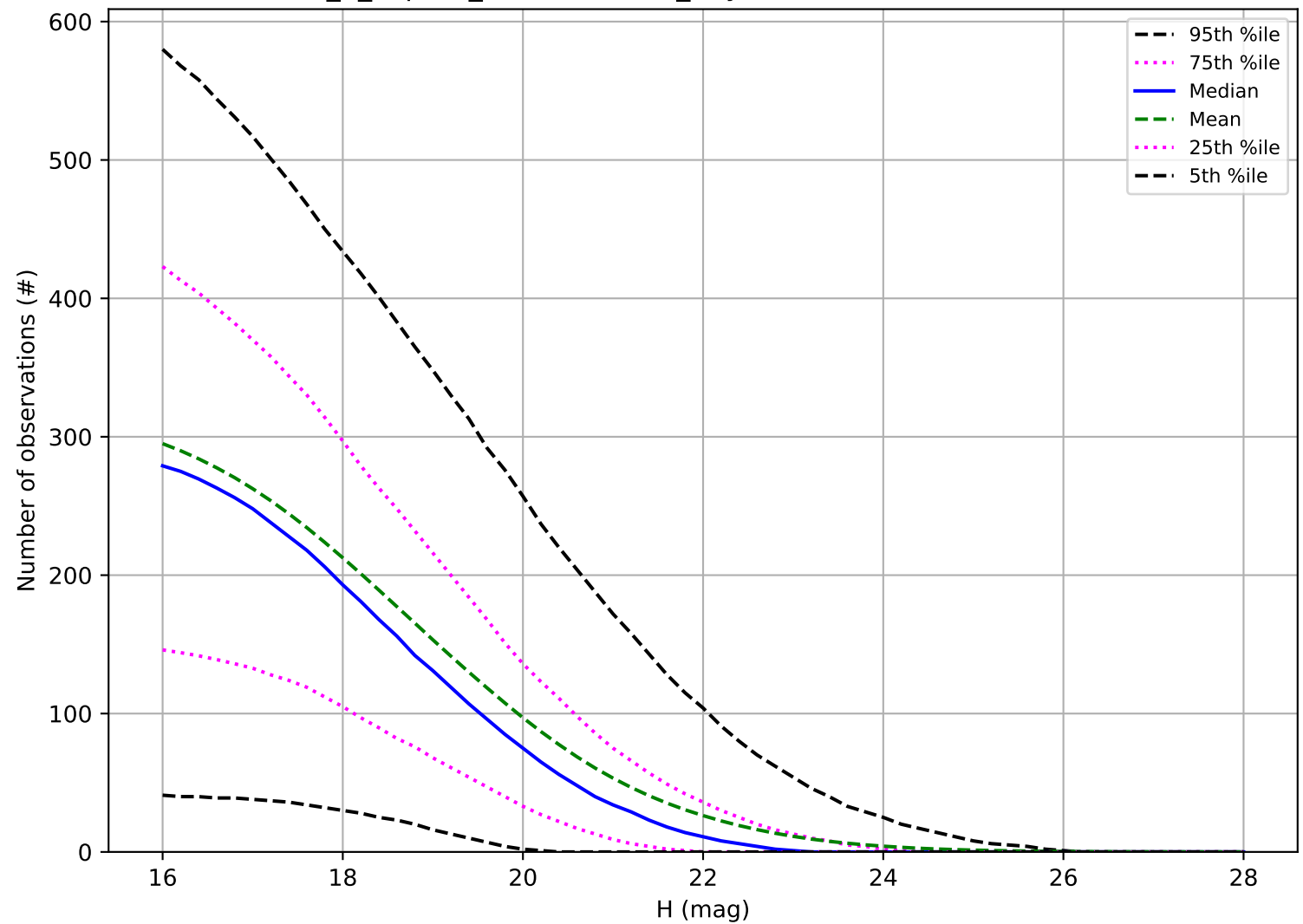
internal_u_expt45_nscale1.0v3.4_10yrs: Number of observations PHA
