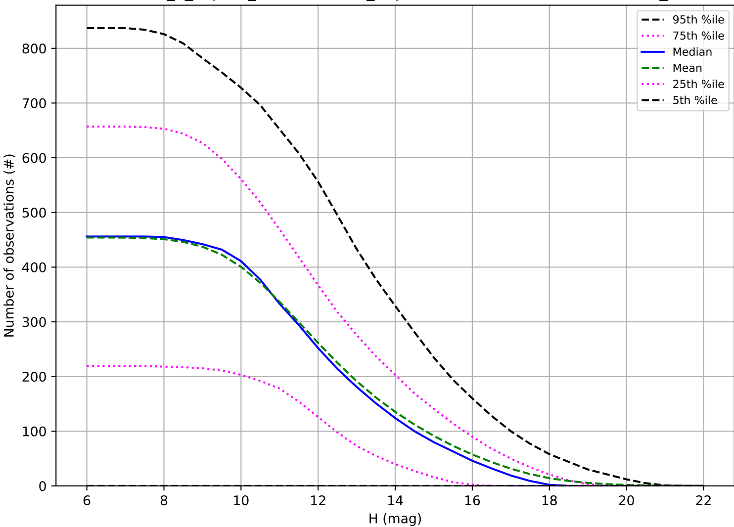
internal_u_expt45_nscale1.0v3.4_10yrs: Number of observations OCC_r5
