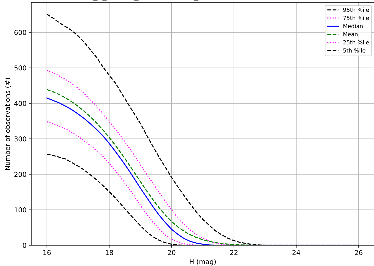
internal_u_expt45_nscale1.0v3.4_10yrs: Number of observations MBA
