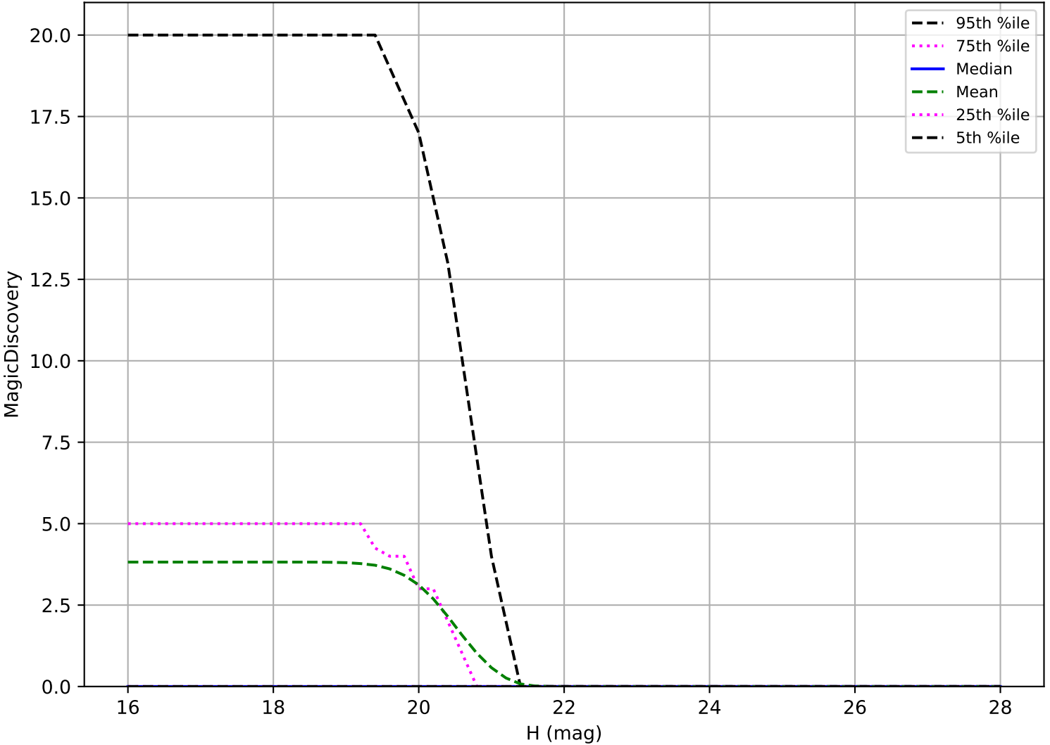
internal_u_expt45_nscale1.0v3.4_10yrs: Vatira 6 detections in 60 nights detection loss
